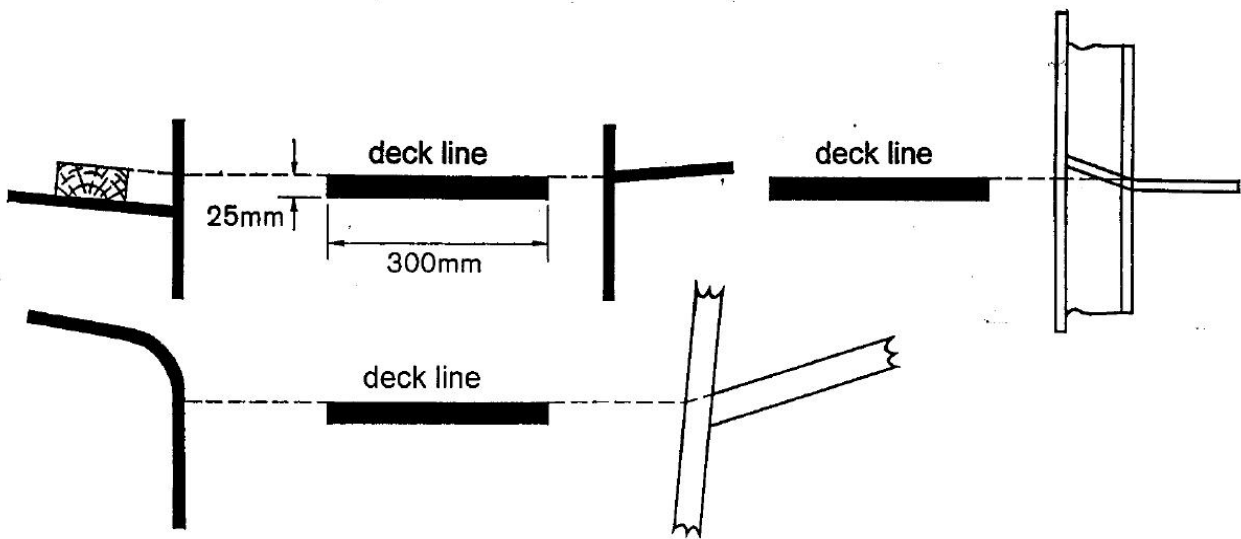
Figure 4.1 Deck line
